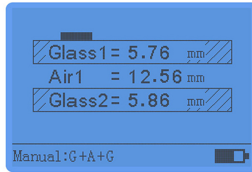
Double glazing
